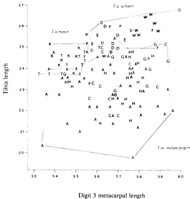
Figure 5 Plot of tibia length versus digit 3 metacarpal length for both adult male and adult female T. m. melanopogon , T. a. achates and T. a. minor for all island populations. Codes for islands are as for Figure 2.
